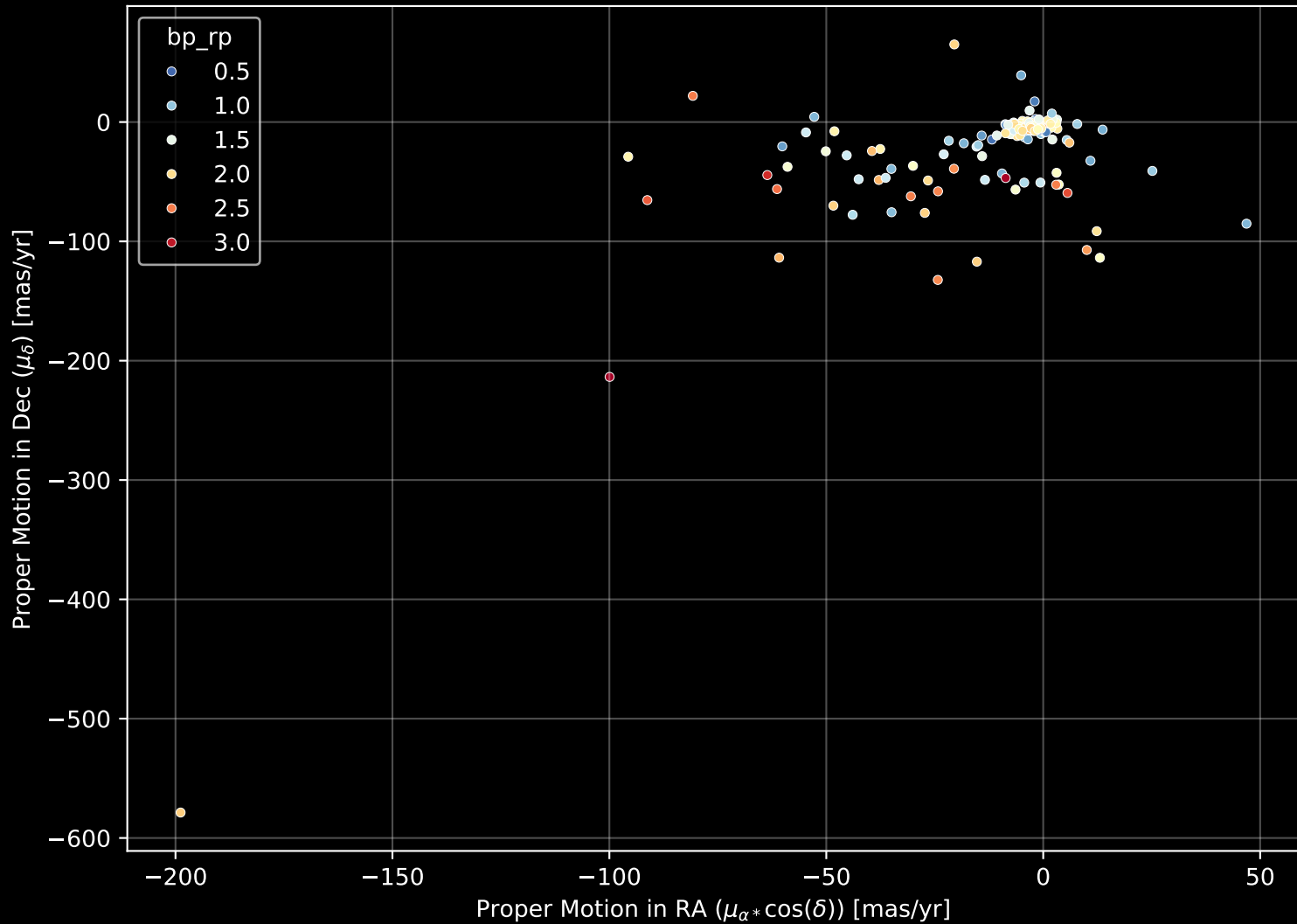
APOGEE DR17 Field: [K2_C11_359+09_btx] Proper Motion Diagram (n= 190)
