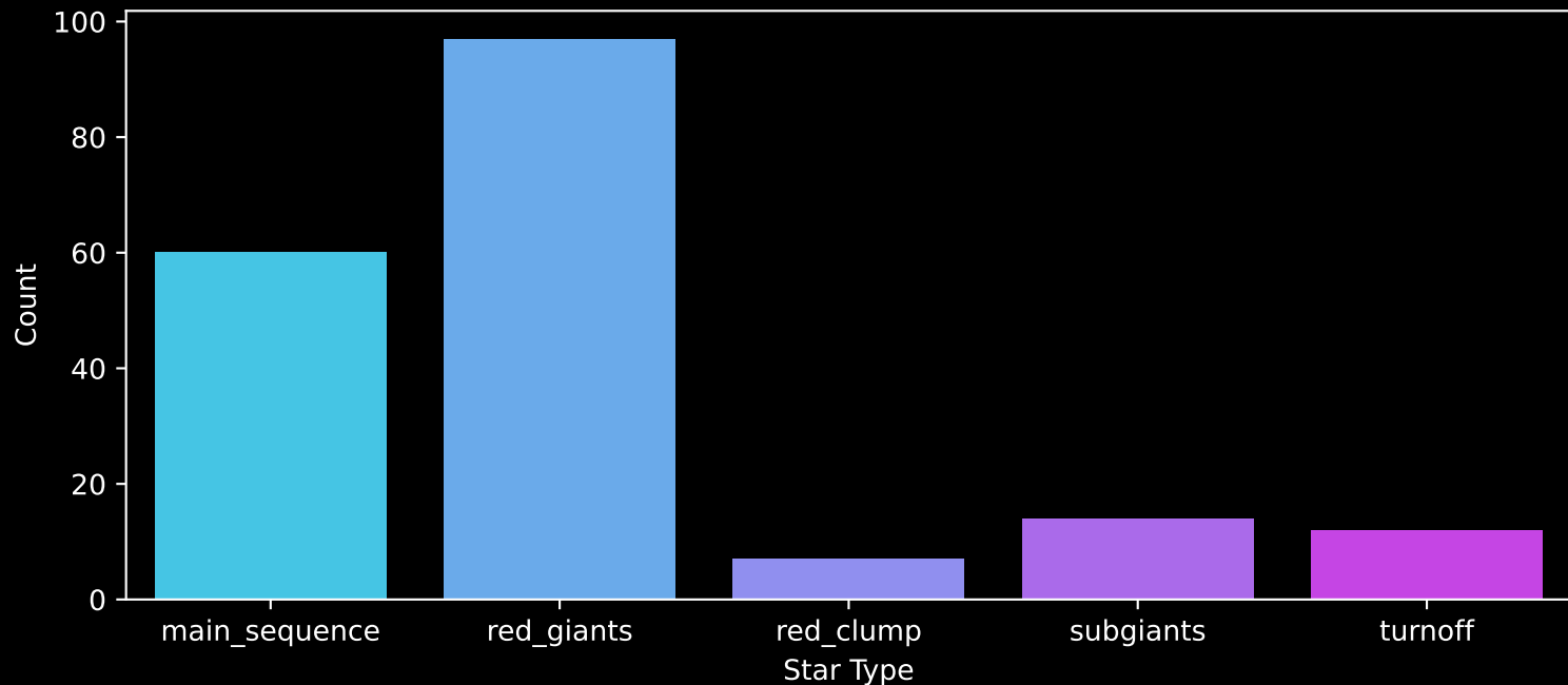
APOGEE DR17 Field: [K2_C11_359+09_btx] Count plot of Star Type
