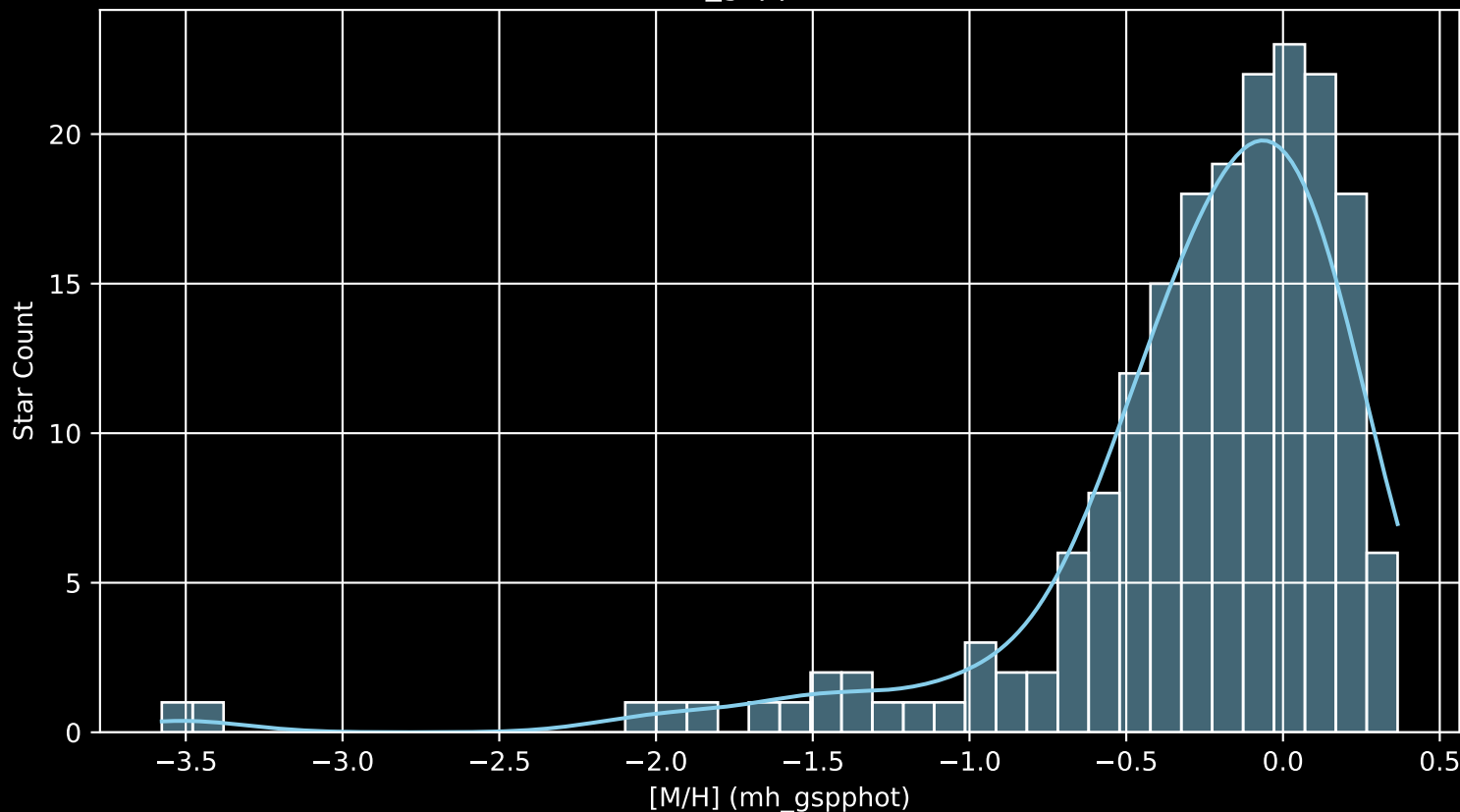
APOGEE DR17 Field: [K2_C11_359+09_btx [M/H] (mh_gspphot) (n= 190)
