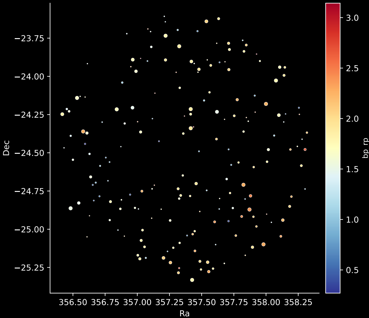
APOGEE DR17 Field: [K2_C11_359+09_btx] Stars: 190
