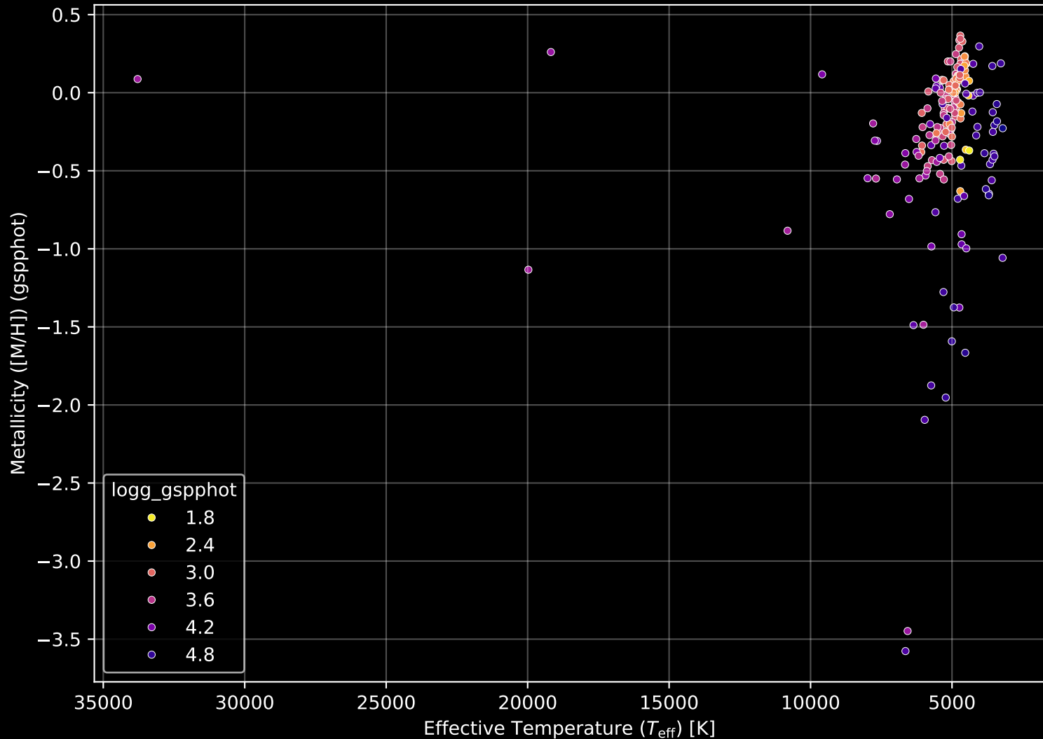
APOGEE DR17 Field: [K2_C11_359+09_btx] Stellar Population Parameters (n= 190)
