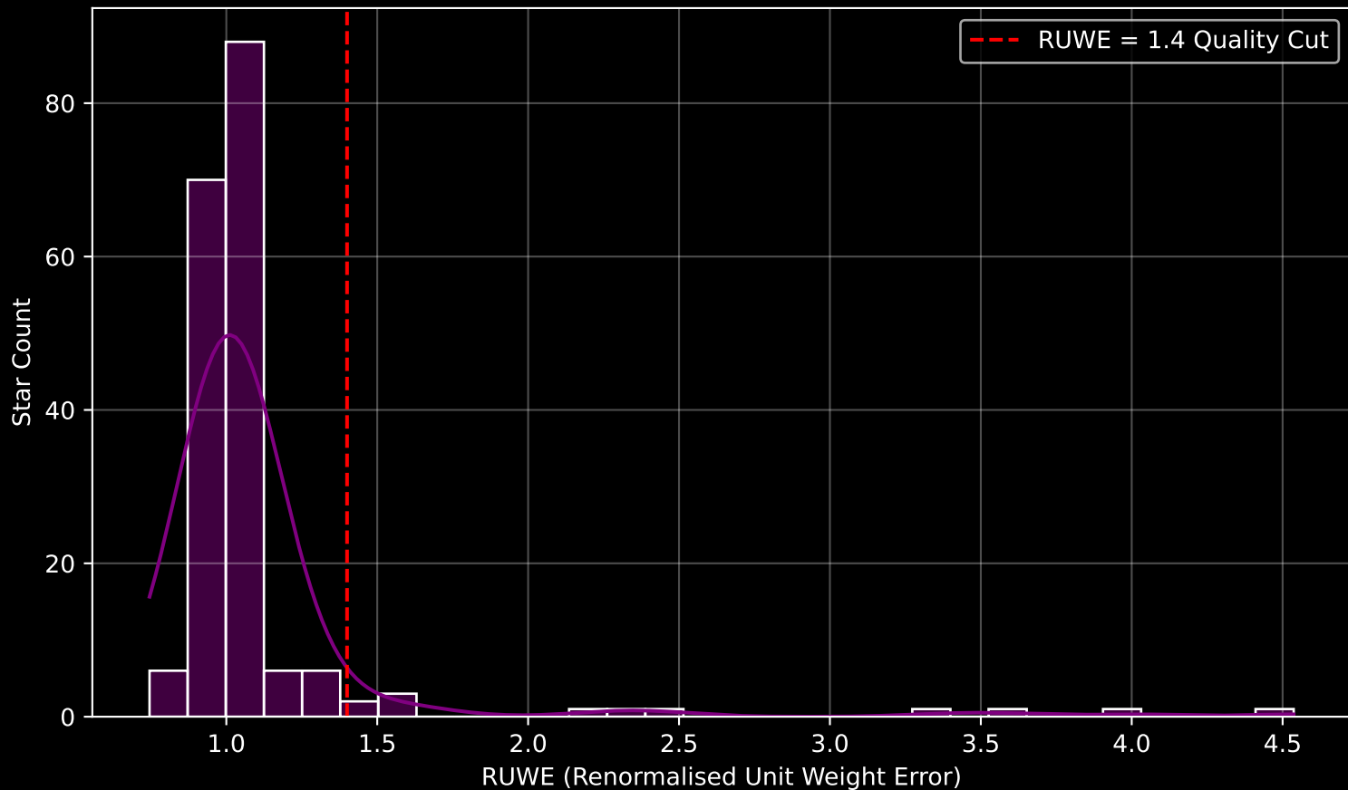
GAPOGEE DR17 Field [K2_C11_359+09_btx] RUWE Distribution (n= 188)
