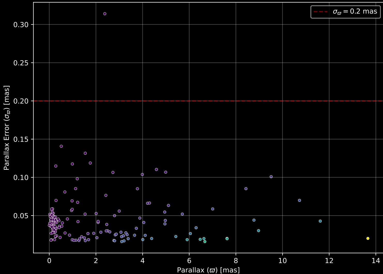
APOGEE DR17 Field: [K2_C11_359+09_btx] Parallax Quality (n= 190)
